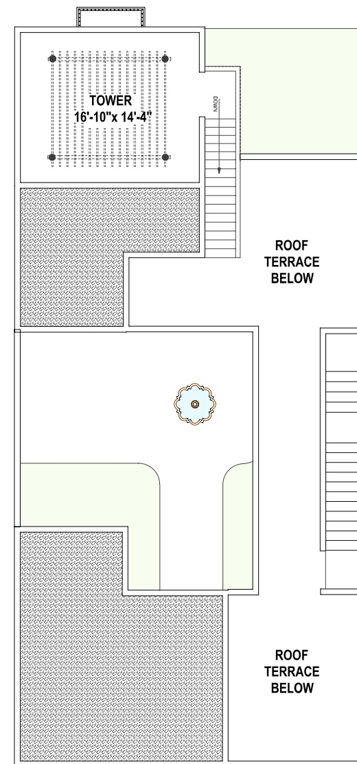
TOWER PLAN
